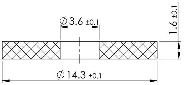
SECTION X-X
