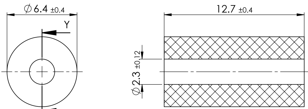
SECTION Y-Y
