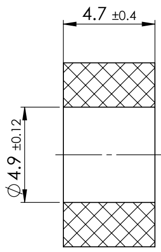
SECTION Y-Y
