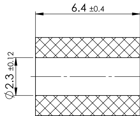
SECTION Y-Y
