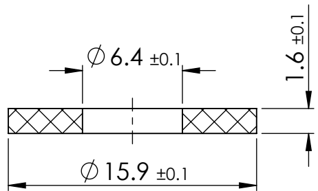
SECTION X-X
