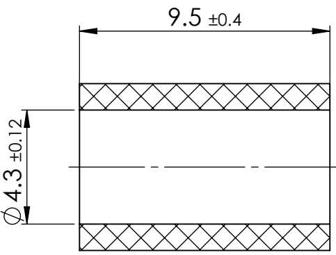
SECTION Y-Y
