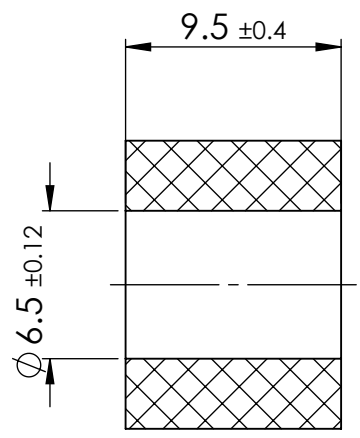
SECTION Y-Y
