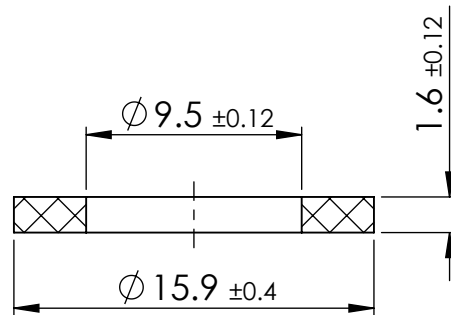
SECTION Y-Y
