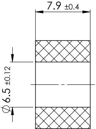
SECTION Y-Y
