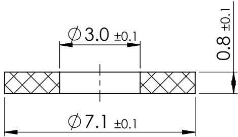
SECTION X-X
