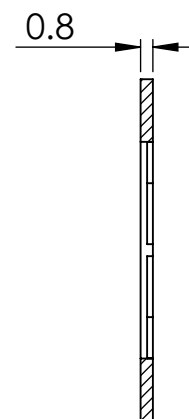
SECTION Y-Y
