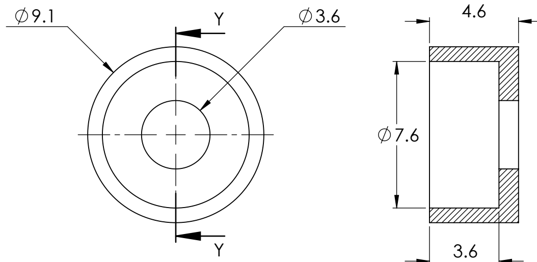
SECTION Y-Y
