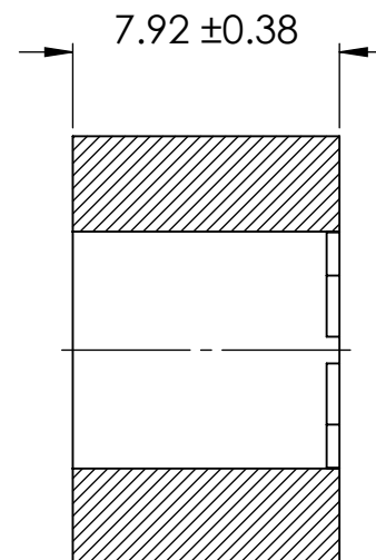
SECTION Y-Y
