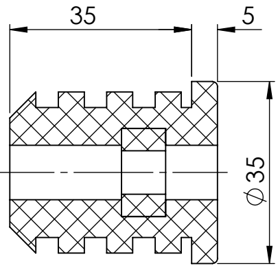
SECTION Y-Y
