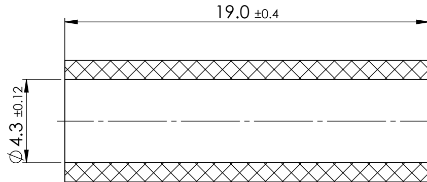
SECTION Y-Y
