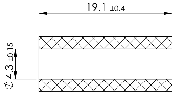
SECTION Y-Y
