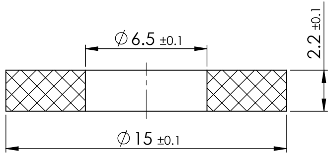
SECTION X-X
