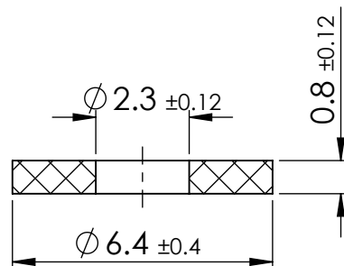
SECTION X-X
