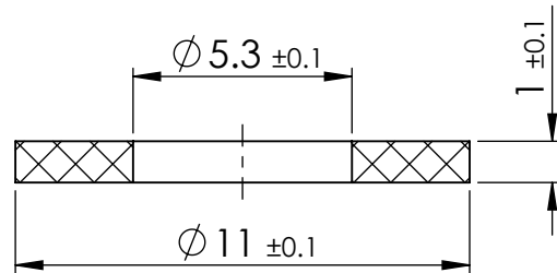
SECTION X-X
