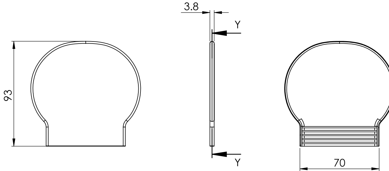
SECTION Y-Y
