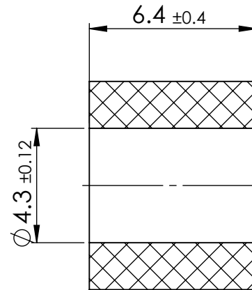
SECTION Y-Y
