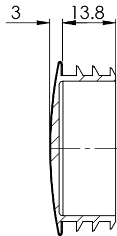
SECTION Y-Y
