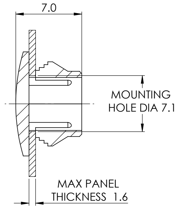
SECTION Y-Y
