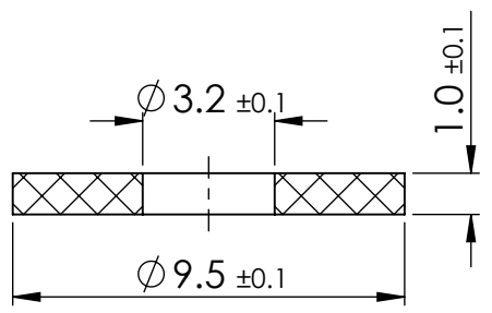
SECTION X-X
