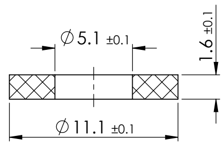
SECTION X-X
