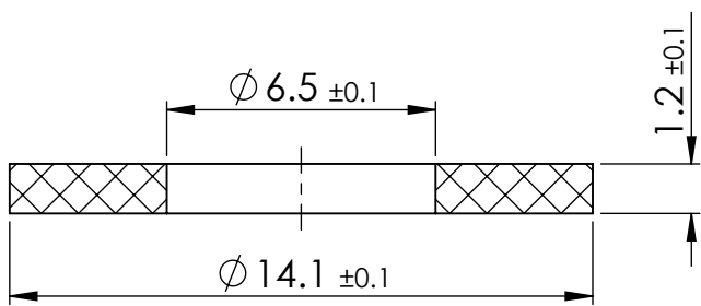
SECTION X-X
