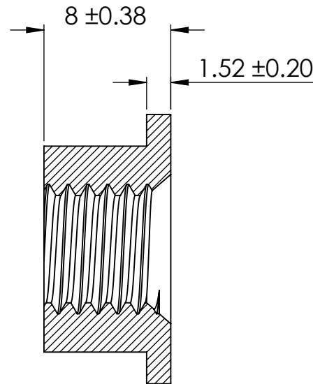
SECTION Y-Y
