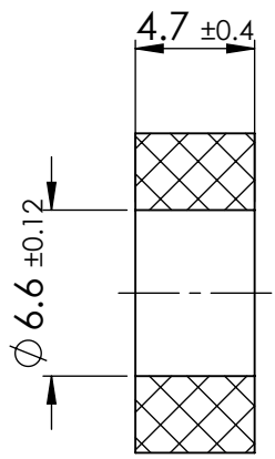
SECTION Y-Y
