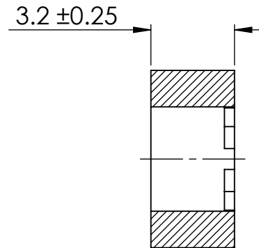
SECTION Y-Y
