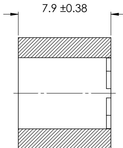
SECTION Y-Y
