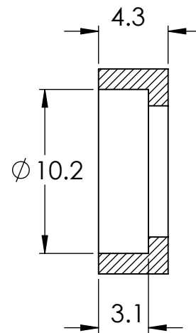
SECTION Y-Y
