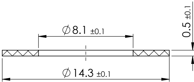
SECTION X-X
