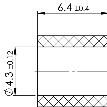
SECTION Y-Y
