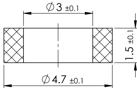
SECTION X-X
