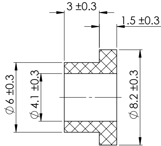
SECTION Y-Y
