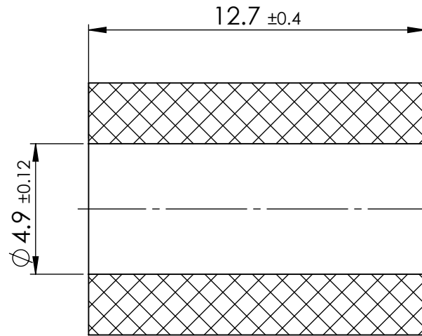
SECTION Y-Y
