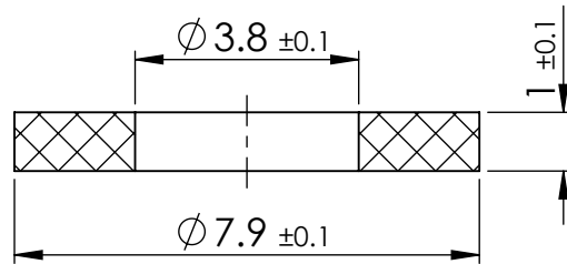
SECTION X-X
