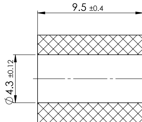
SECTION Y-Y
