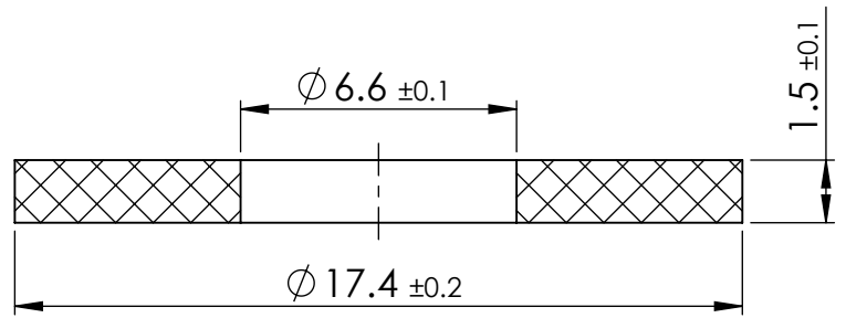
SECTION X-X
