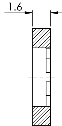
SECTION Y-Y
