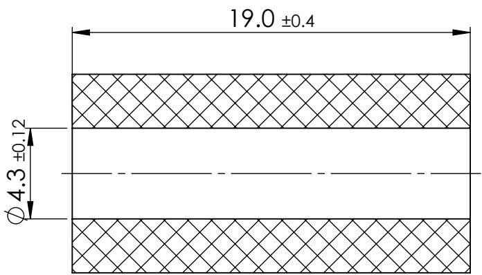
SECTION Y-Y
