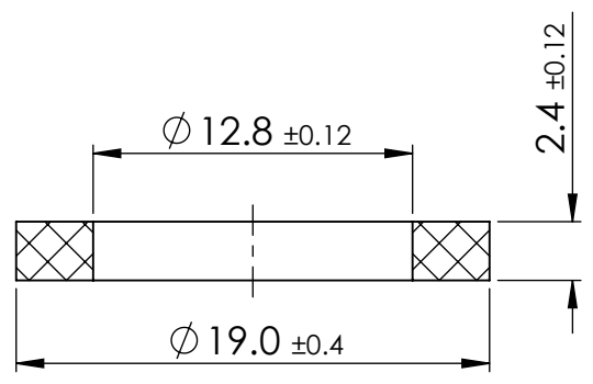
SECTION Y-Y
