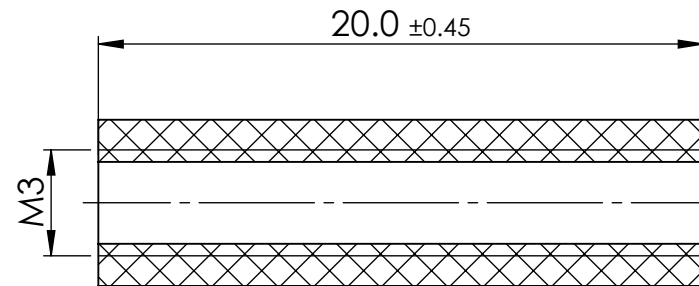
SECTION Y-Y
