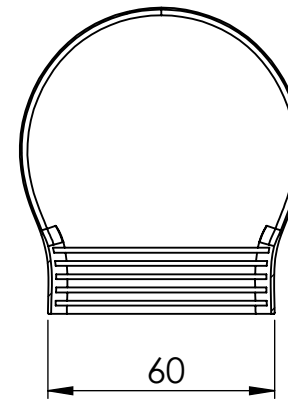
SECTION Y-Y
