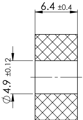
SECTION Y-Y
