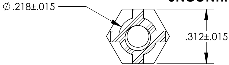
SECTION B-B
