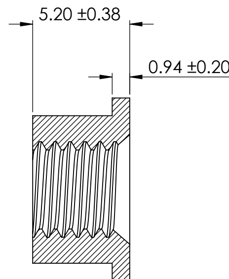
SECTION Y-Y
