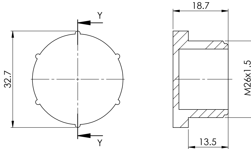
SECTION Y-Y
