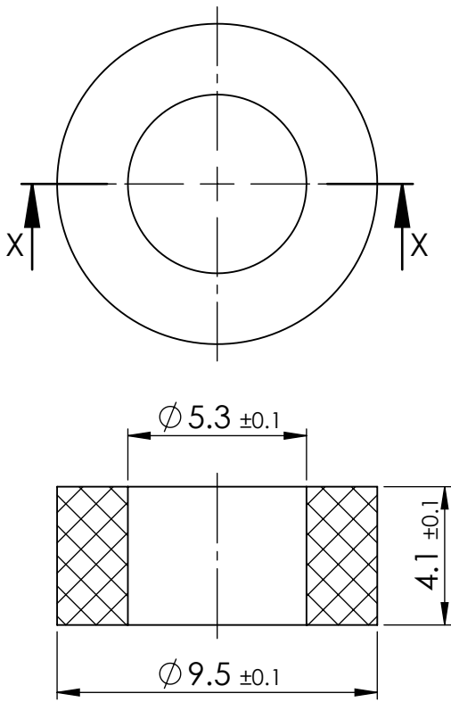
SECTION X-X
