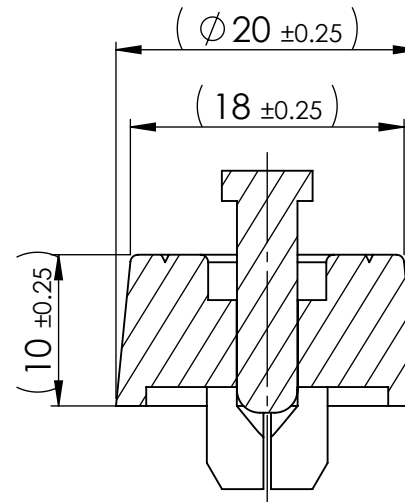
SECTION Y-Y
